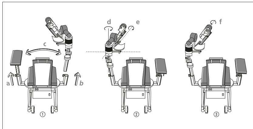
Ombouwschema ARTROMOT®-E2:
